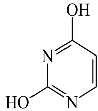
2,4-diossi-pirimidina
