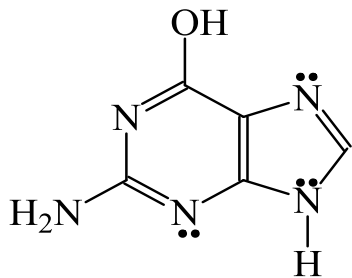
guanina
